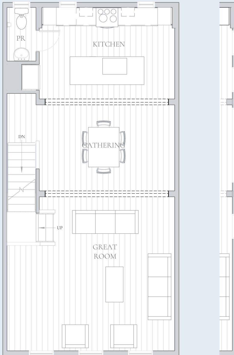
First Floor Ceiling Height 9'-0"
