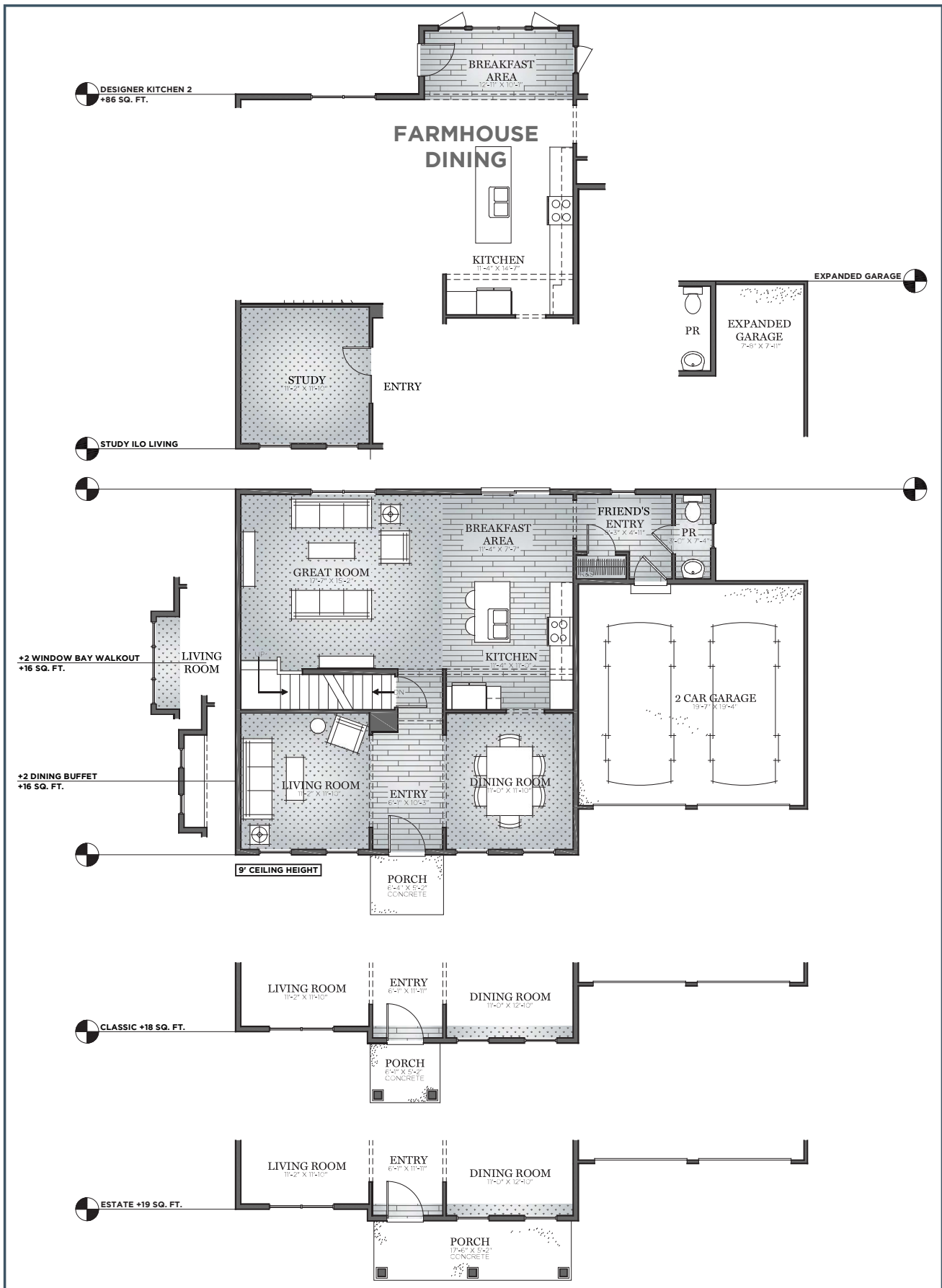
FIRST FLOOR MODIFY FLOOR PLAN OA DIMENSION 50 X 37
